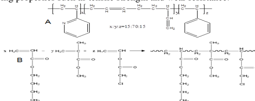
Fig 5. (A) Styrene butadiene-vinyl pyridine copolymer (SBV). (B) Copolymerization of BA, MMA and VCA (preparation of ACM rubber)
