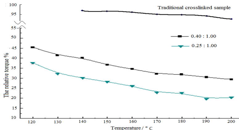
Fig 7. Temperature dependence of the relative torque of the crosslinked SBV rubber filled with reactive filler [63].
