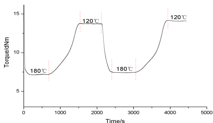
Fig 9. Thermo-reversible cycle of chloro-functionalized PSt filler cross-linked SBV [63].
