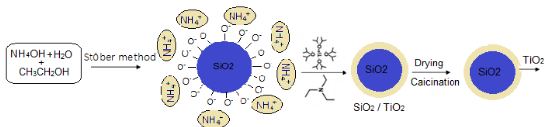
Fig 3. Nitrogen-doped SiO 2 /TiO 2 inorganic-inorganic core-shell nanoparticles .
