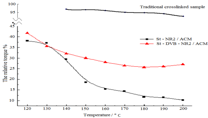
Fig 6. Temperature dependence of the relative torque of the crosslinked ACM rubbers filled with amino-functionalized PSt particles and DVB crosslinked amino-functionalized PSt particles [86].
